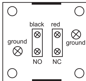
cabl e entry gland PG13,5
